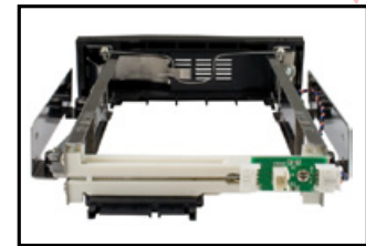
Rear Connector
